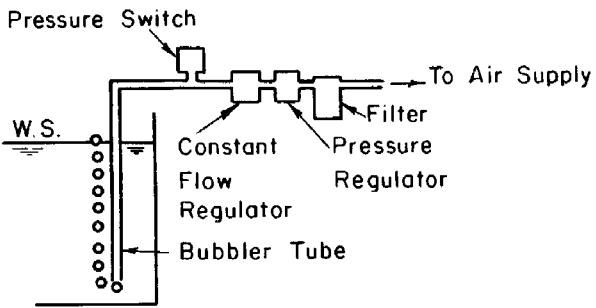
BUBBLER CONTROL
