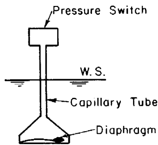
DIAPHRAGM CONTROL
