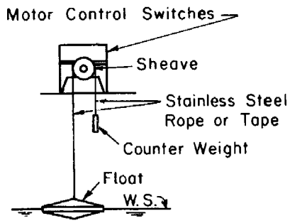
FLOAT CONTROL
