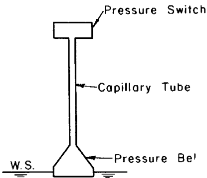
BELL CONTROL
