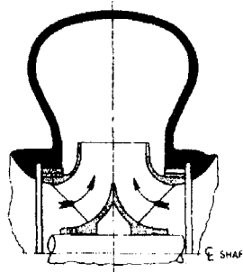
Radial Flow Pump (Double Suction)
