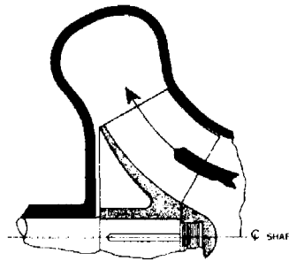
Mixed Flow Pump
